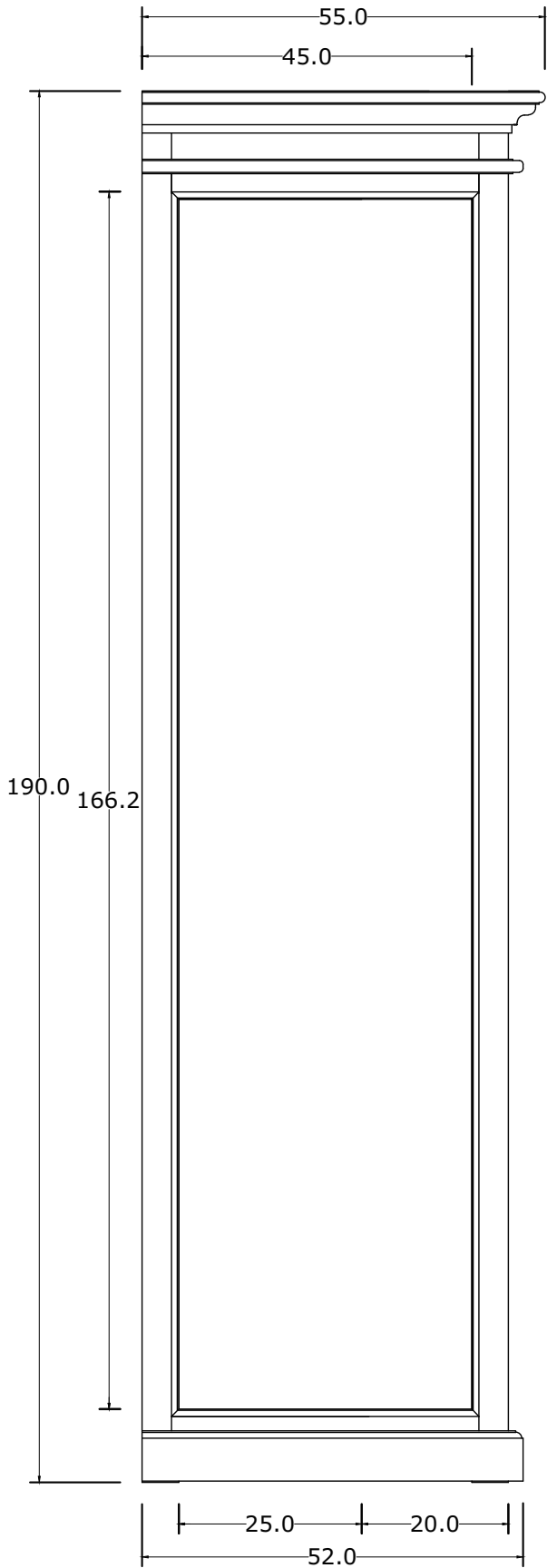
SIDE VIEW
