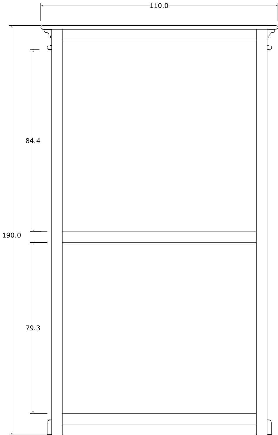
BACK VIEW
